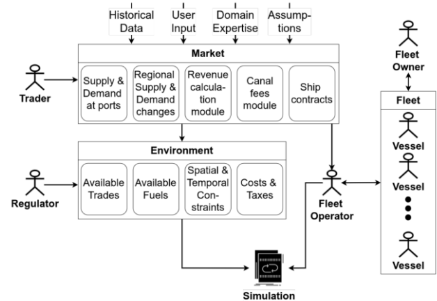
FIGURE 4: A PRINCIPAL SCHEME OF THE ABM FRAMEWORK BY BUERMANN ET AL. [39].
